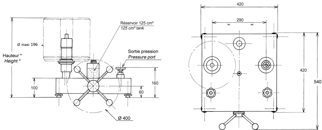
Height with standard set of weight : (bar, KPa) : 4300 mm (PSI) : 540 mm Unit used : mm
